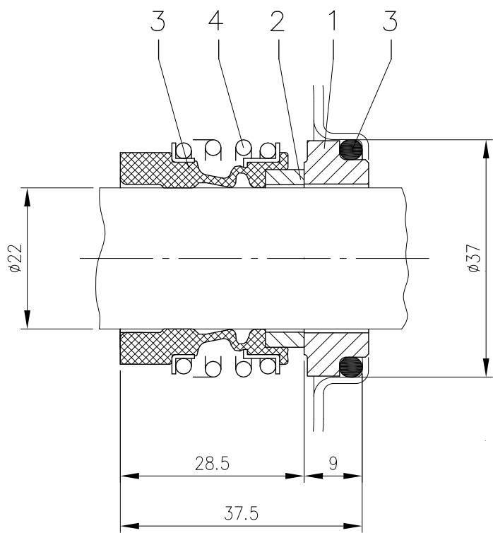
MECHANICAL SEAL (HS version)
