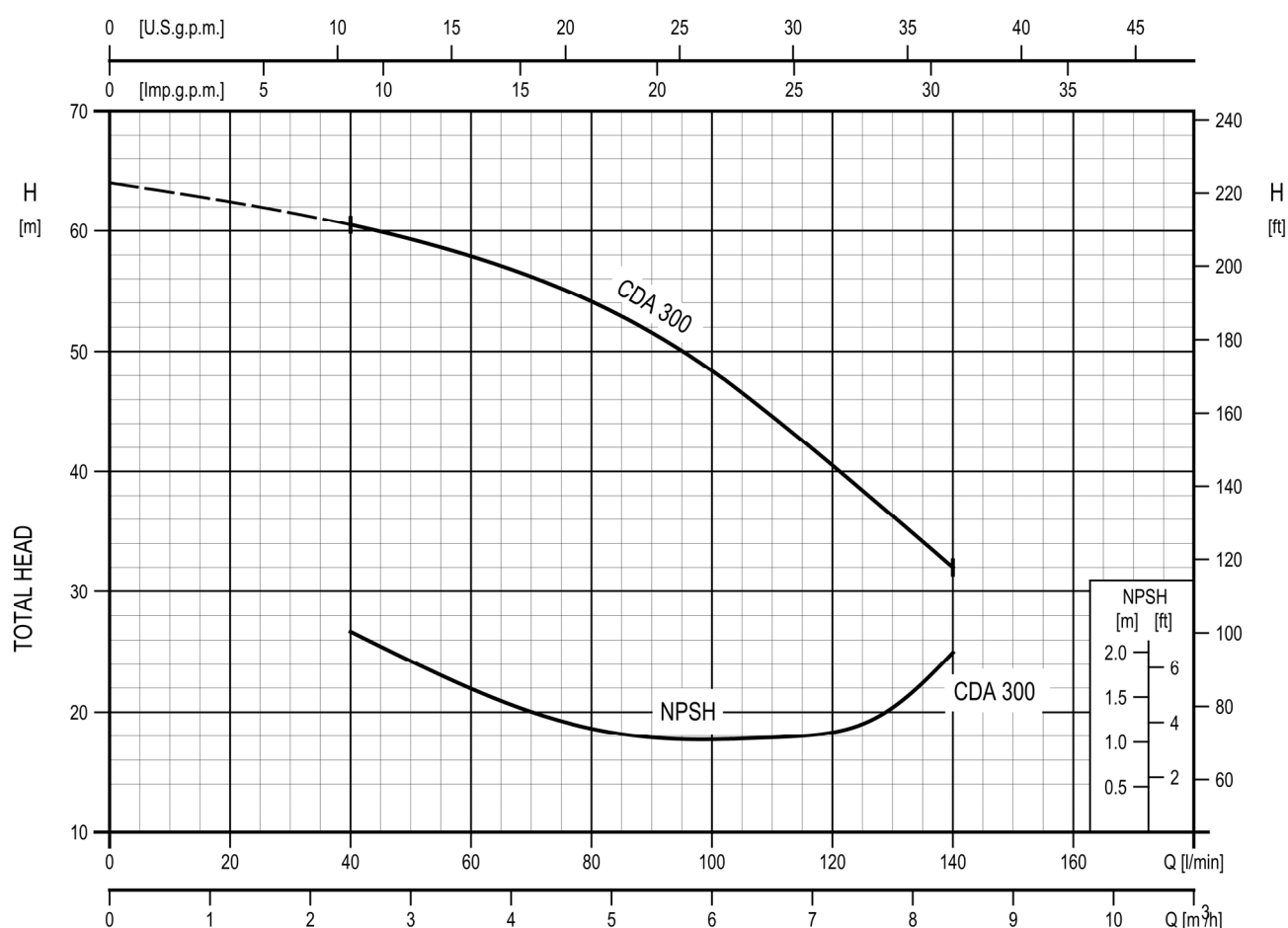
CDA 3.00 - Impeller diameter = 156 mm
